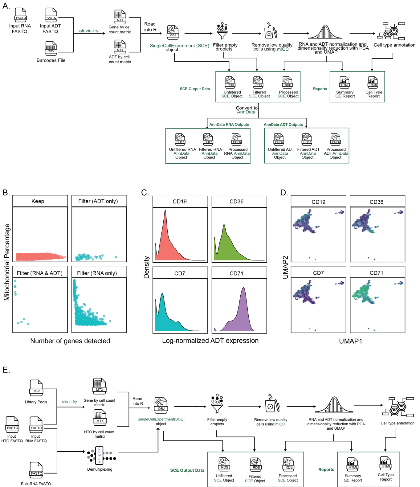
Figure S2: Processing additional single-cell modalities in scpca-nf .
